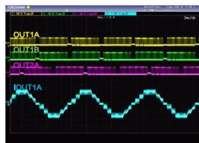
Figure 17. QUARTER STEP 駆動波形 (CLK : 2400Hz)
